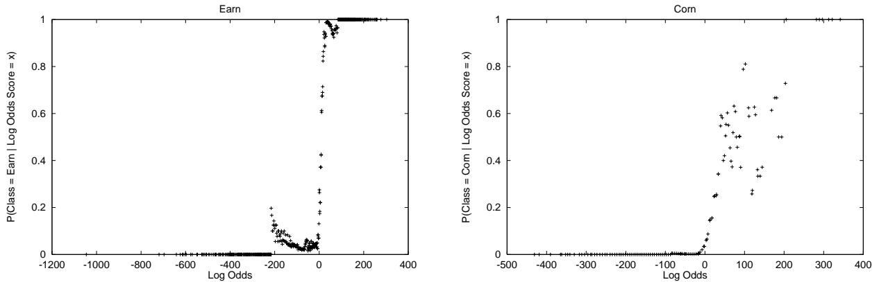
Figure 3: Posterior Distribution given Log Odds Scores for Earn and Corn Binary Classifiers
