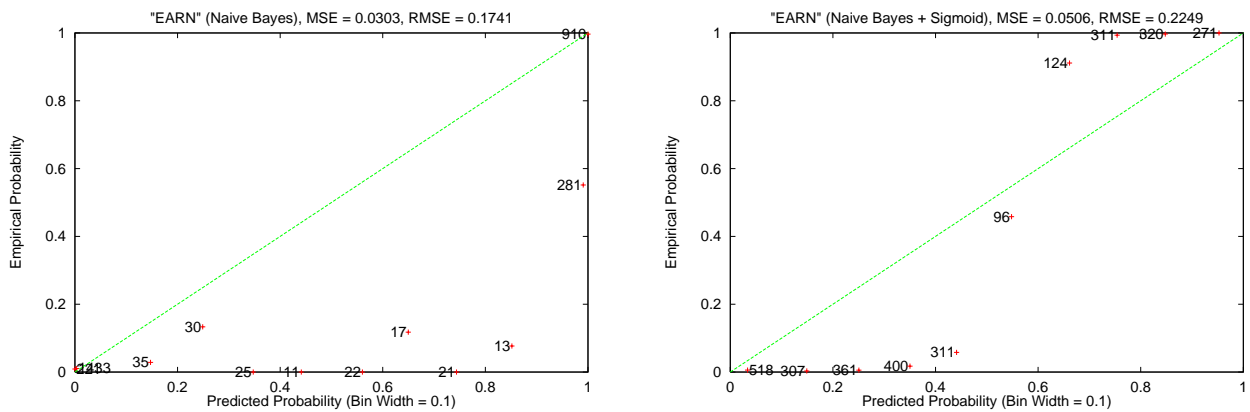
Figure 5: Reliability Diagrams for Class “Earn”
