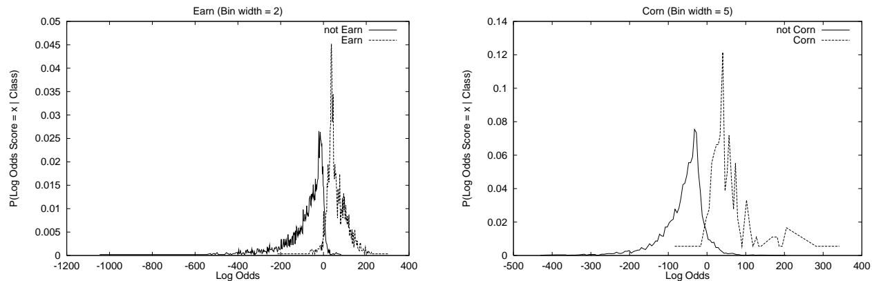
Figure 2: Conditional Distribution of Log Odds Scores for Earn and Corn Binary Classifiers
