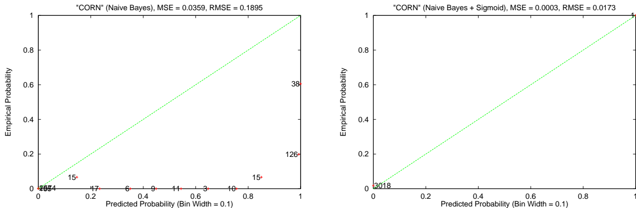
Figure 6: Reliability Diagrams for Class “Corn”
