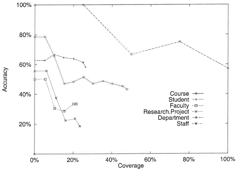
Figure 5: Accuracy/coverage tradeoff for hyperlink classifiers.
