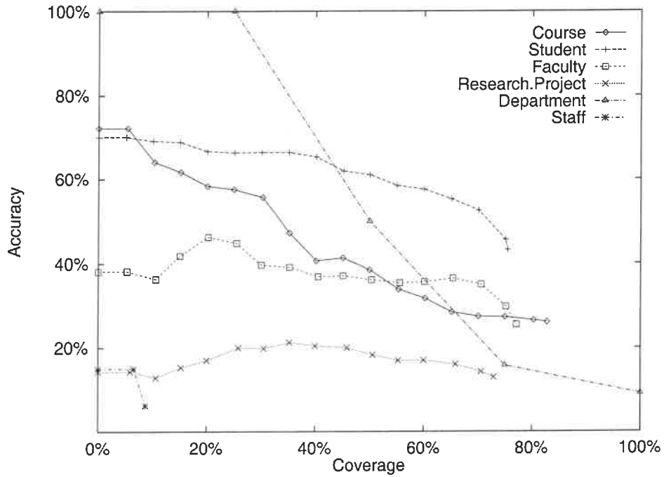
Figure 4: Accuracy/coverage tradeoff for full-text classifiers. Predictions within each class are ordered according to their confidence. Each curve shows the behavior of the classifier as a threshold on this confidence is varied. The x -axis represents the percentage of pages for a given class that are correctly classified as belonging to the class. The y -axis represents the percentage of pages assigned to a given class that are actually members of that class.
