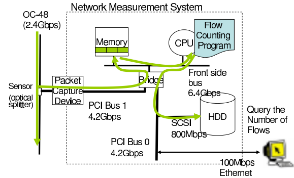
Figure 1: Continuous Monitoring System
