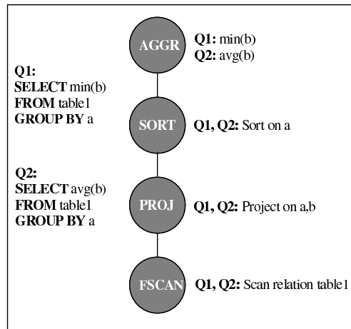
Figure 3. Two "mergeable" query plans
