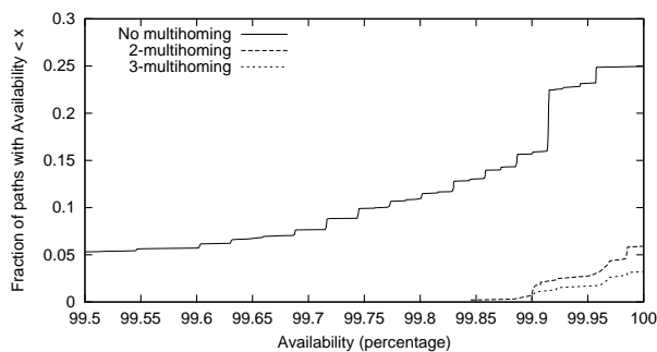
Figure 13: End-to-end failures: Distribution of the availability on the end-to-end paths, with and without multihoming. The ISPs in the 2- and 3-multihoming cases are the best 2 and 3 ISPs in each city based on RTT performance, respectively. k -Overlay routing, for any k , achieves 100% availability and is not shown on the graph.
