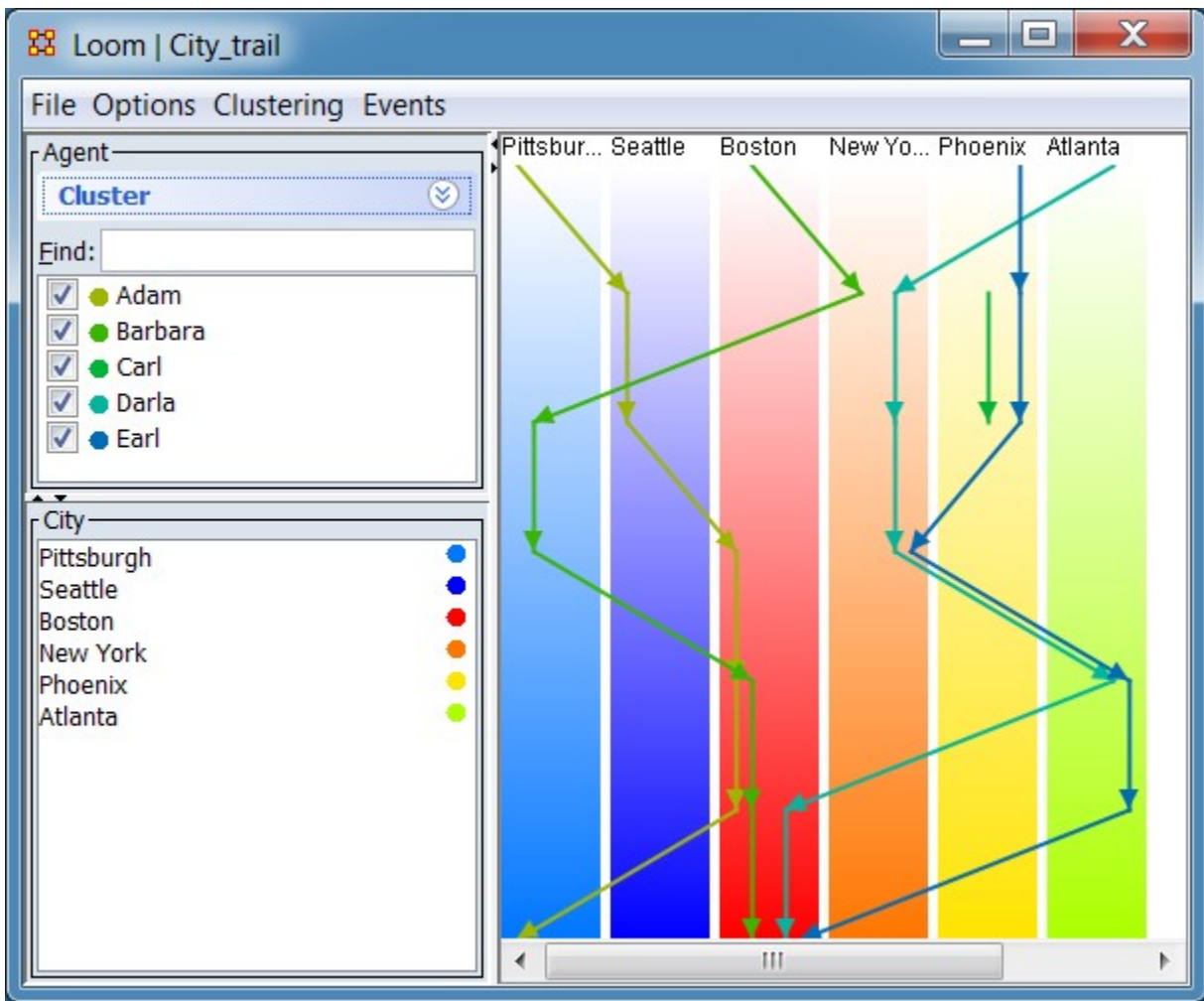
Trail visualization of city to city movement from trails dynamic meta-network covering a one-week period.
