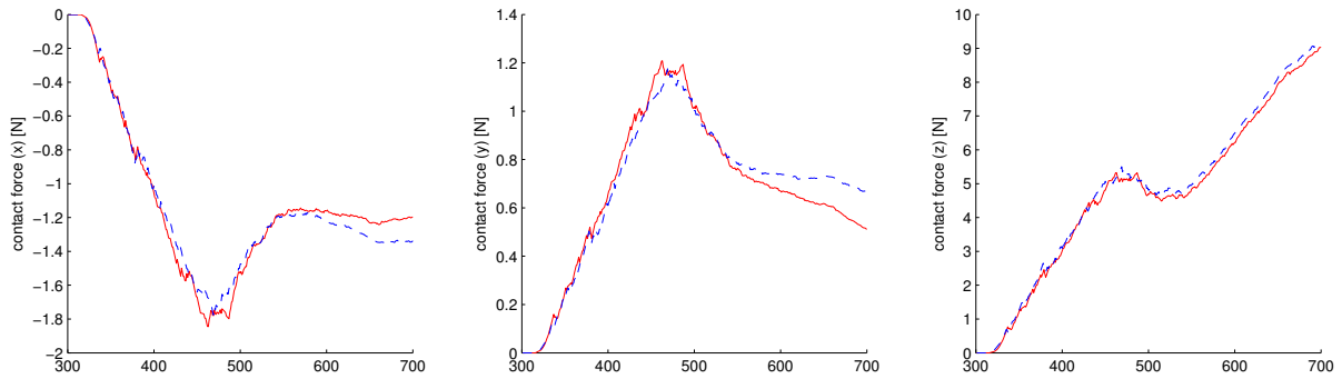
Figure 3.30: Asymmetric contact (detailed plot for shallow penetrations): the contact forces are not symmetric, however the difference is small for shallow penetrations. Same notation as in Figure 3.29. X -axis corresponds to sample indices.
