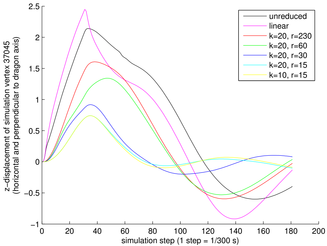
Figure 2.21: Trajectory of a selected vertex: Z-displacement (i.e., horizontal and perpendicular to main dragon axis) of simulation vertex where force load was applied in the “back” sequence (Figure 2.20).
