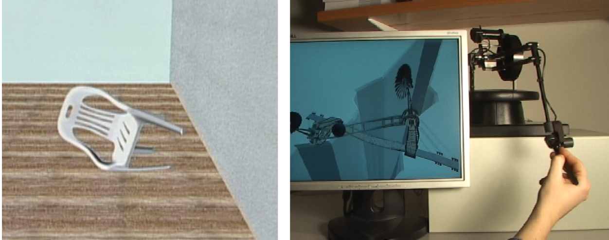
Figure 3.22: Haptic contact between reduced deformable objects and rigid objects modeled by simple analytical functions: Left: The user-manipulated deformable chair is a deformable pointshell with about 26,000 vertices, rendered against an analytical implicit function of two perpendicular walls. Right: The deformable bridge is a deformable pointshell of about 41,000 vertices, rendered against a user-manipulated sphere. The chair is a linear reduced deformable model (linear modal analysis deformations). The bridge is a nonlinear StVK reduced deformable model, as described in the first part of the thesis.
