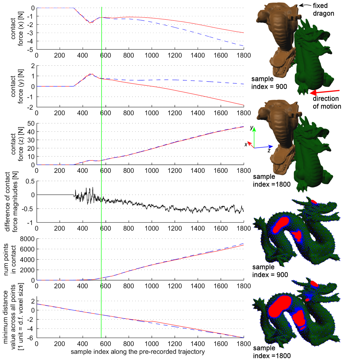
Figure 3.29: Asymmetric contact model: The contact force changes under role reversal, however the error is quite reasonable. The first contact case (green dragon=pointshell, brown dragon=signed distance field) is depicted with a solid red line, the reverse case (green dragon=signed distance field, brown dragon=pointshell) is shown in dashed blue. Both lines show the raw contact force on the green (i.e., moving) dragon. The top-right image shows the configurations at samples 900 and 1800, respectively. The bottom-right images depict points in contact (red=in contact, blue=traversed by tree, but not in contact). Note that the z -axis is aligned with the direction of motion, and is (about) normal to the contact areas; z -force is therefore the normal contact force and is as such substantially larger than tangential forces. Penetration depths are large in this experiment; in our simulations, virtual coupling coupling saturation would prevent penetrations deeper than about 1 voxel. The vertical green line denotes the sample index where penetration reaches 1 voxel.
