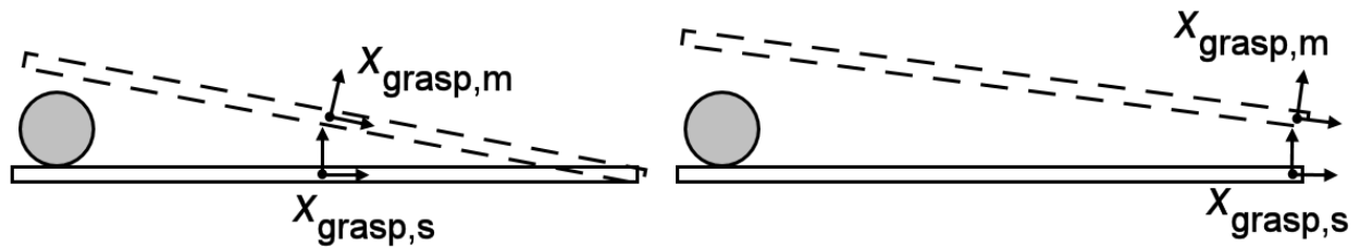
Figure 4.1: Grasping location affects virtual coupling forces and torques: The user is manipulating this long pole against a rigid obstacle (a cylinder viewed from top), and will feel different forces and torques depending on the choice of X_{\text{grasp}} (Left: at pole center, Right: at pole far end). Stippled line denotes the manipulandum and solid line denotes the simulation object. Virtual coupling tries to align the two coordinate systems.
