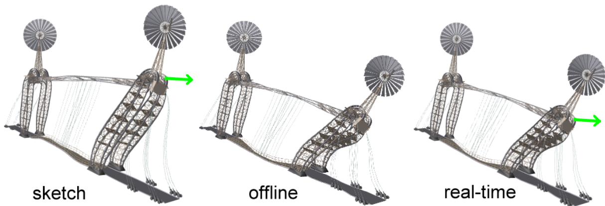
Figure 2.11: Basis from Sketch: Left: User interacts with a linear model. Resulting shape is distorted. Center: Applied force is recorded and sent to an unreduced offline static solver to solve for the corresponding nonlinear shape. Several such shapes are then processed by mass-PCA to obtain a basis of motion. Right: If same force is re-applied during the reduced runtime simulation, a shape which is visually almost indistinguishable from the center image emerges.
