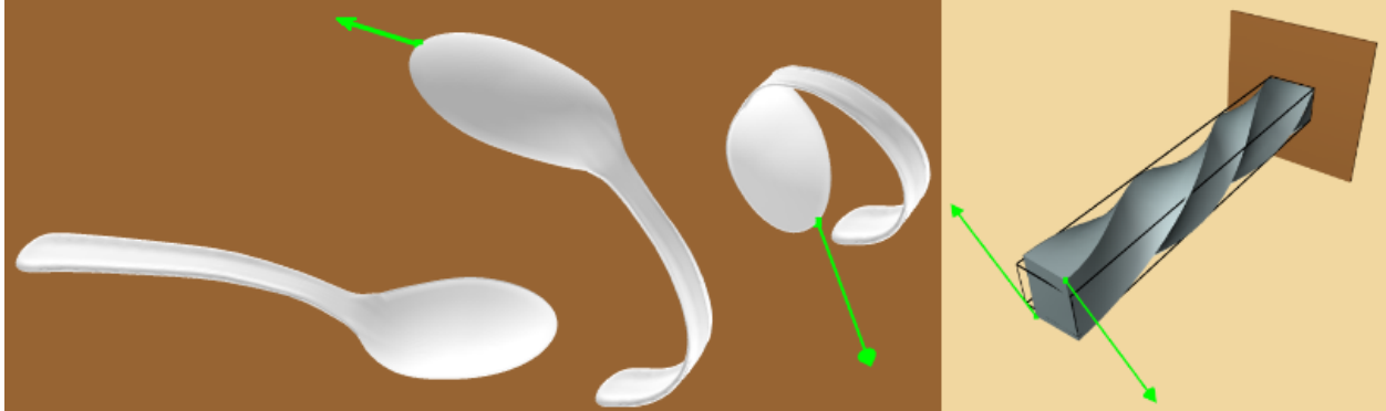
Figure 2.14: Extreme shapes captured by modal derivatives: Although modal derivative are computed about the rest pose, their deformation subspace contains sufficient nonlinear content to describe large deformations. Left: Spoon ( k = 6, r = 15 ) is constrained at far end. Right: Beam ( r = 5 , twist angle= 270^\circ ) is simulated in a subspace spanned by “twist” linear modes and their derivatives \Psi^4, \Psi^9, \Phi^{44}, \Phi^{49}, \Phi^{99} .
