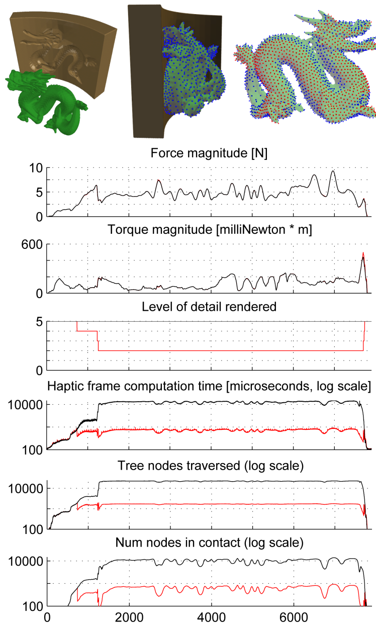
Figure 3.28: Graceful degradation supports large conforming contacts to allow time-critical approximation of very difficult contact configurations (here under 1 millisecond). Top Left: A dragon “peg” inserting into a matching dragon “hole” obtained via CSG difference. Top Middle: dragon manipulated haptically into the hole. Top Right: Large contact area with traversed points in blue (43% of all L2 points), and contacting points in red (21% of all L2 points). (Bottom Graphs) Simulation data for a pre-recorded manipulandum trajectory is rendered in two ways: using GD ( in red ) with warm threshold at 2000 nodes; without GD (in black) with all five tree levels. Same machine as in Table 3.1. The common x -axis corresponds to haptic frames.
