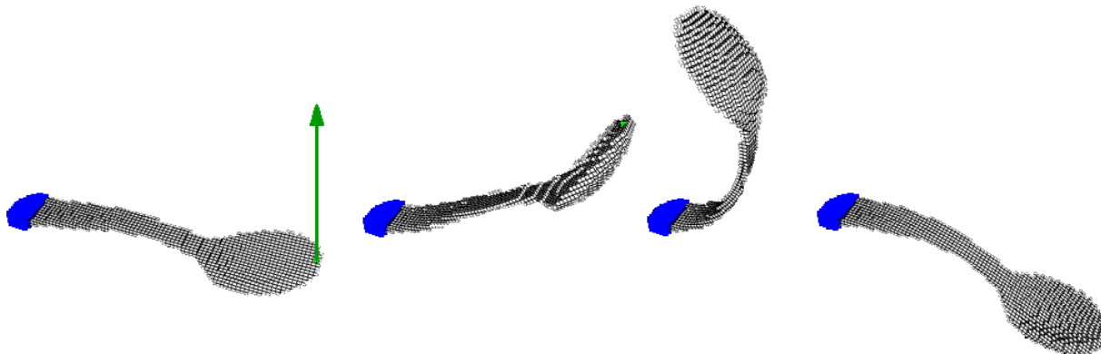
Figure 2.2: Nonlinear FEM simulation of a voxelized elastic spoon: The spoon consists of 2005 elements (voxels in this case) and has 11,094 degrees of freedom. Motion was computed using an unreduced approach: direct internal force and stiffness matrix evaluation, combined with the implicit Newmark timestepping scheme and a conjugate gradient solver. Spoon is constrained at the far end (blue), and the motion is induced by a short initial vertical impulse (green). Left-most picture is the rest pose, followed by three representative frames of the dynamic simulation (free vibration).
