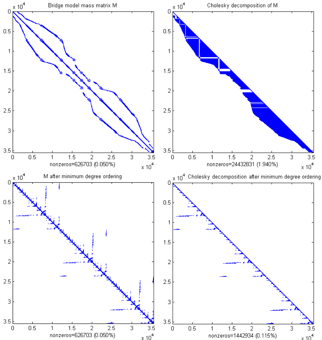
Figure 2.10: Mass matrix Cholesky decomposition (bridge model, 11,829 simulation vertices): Top-left: non-zero entries in the original mass matrix M (mesh generated via squashing cubes); Top-right: Cholesky factor of M ; Bottom-Left: Permuted mass matrix (minimum degree ordering permutation); Bottom-Right: Cholesky factor of the permuted mass matrix.
