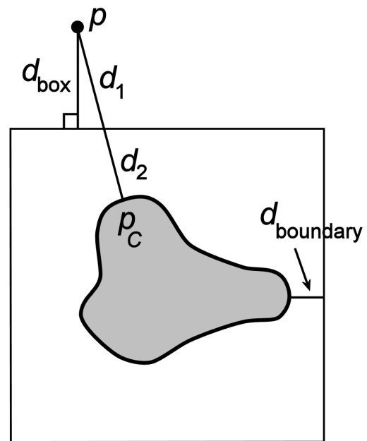
Figure 3.21: The proof of Inequality 3.14.
