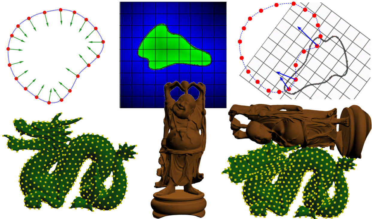
Figure 3.6: Point-contact model: Left: Pointshell with inward normals. Middle: the signed distance field. Right: deformable contact and contact forces.
