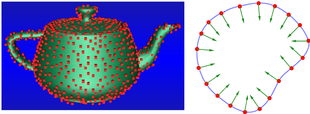
Figure 3.2: VPS pointshell : Left: the pointshell points for the teapot model. Right: a schematic representation of the pointshell, with inward normals. Both images are from [MPT99].
