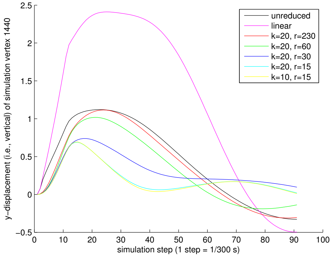
Figure 2.19: Trajectory of a selected vertex: Vertical displacement of simulation vertex where the force load was applied in the “head” sequence (Figure 2.18).
