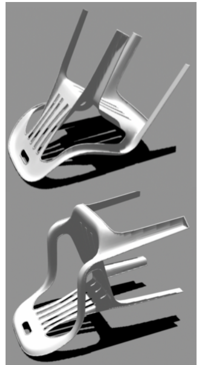
Figure 3.9: Normals obtained only from the chair geometry will give contact forces in the wrong direction for one of the two chair orientations.
