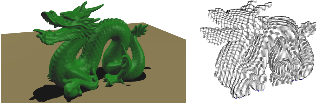
Figure 2.17: The dragon model: Left: the rendered dragon model in the rest configuration. Right: simulation voxel mesh. Bottom vertices are fixed rigidly.
