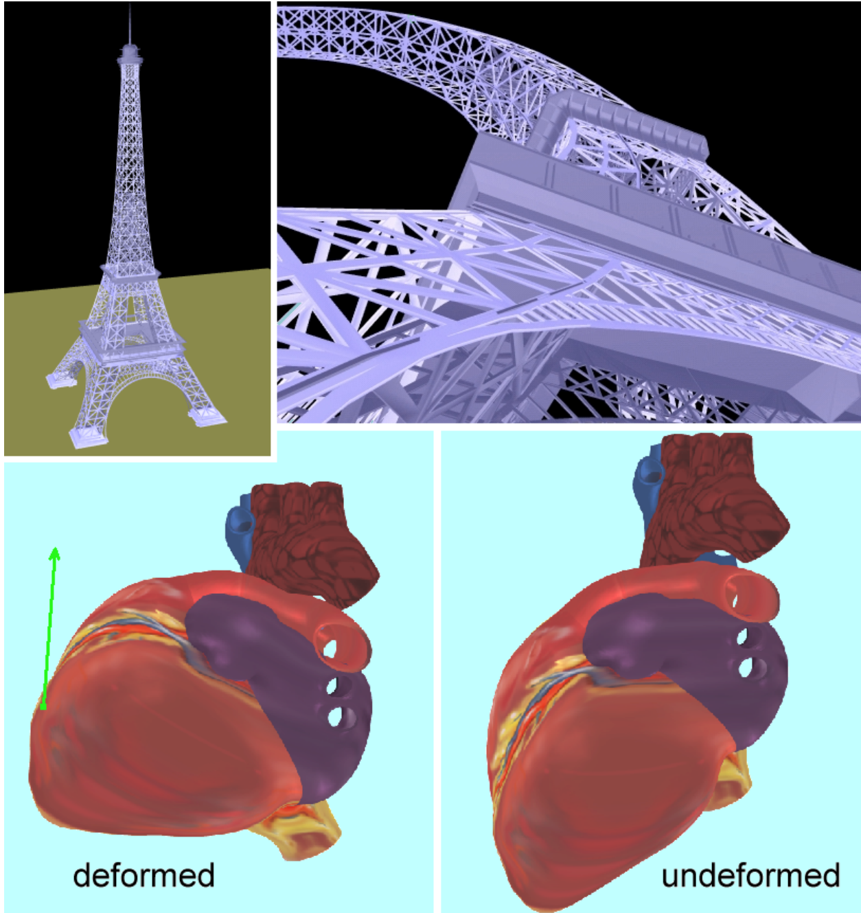
Figure 2.5: Subspace integration of Eiffel tower and heart models
