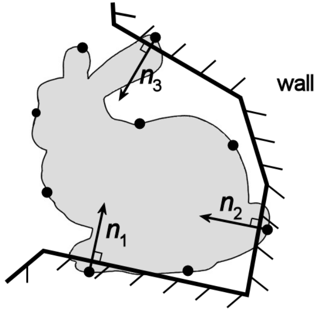
Figure 4.4: Multiplane penalty contact ( \ell = 3 ).
