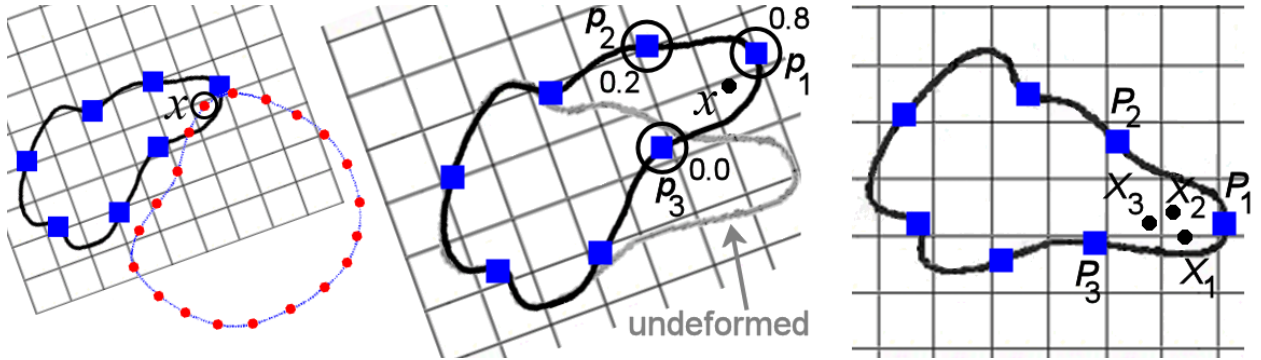
Figure 3.23: Deformed distance field approximation: Left: Proxies (squares), the query pointshell point at x . Middle: 3-nearest neighbors and their weights. Right: material configuration pull-backs X_i of x .
