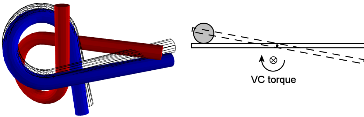
Figure 4.5: Virtual coupling torque saturation: Left: without torque saturation, the user can squeeze the blue alpha in between the other (red) alpha's gap, by using the blue alpha's long end as a lever. Right: A fixed torque saturation limit will overpower contact penalty forces for long objects, such as for this manipulated long (horizontally positioned) rod in contact with a static vertical cylinder (view from top).
