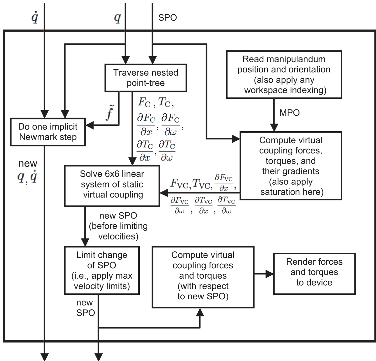
Figure 4.2: Block diagram of one haptic cycle: SPO=Simulation object Position and Orientation, MPO=Manipulandum Position and Orientation.
