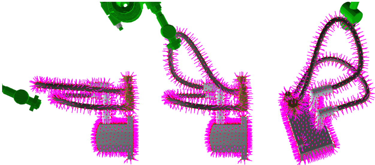
Figure 3.7: Dynamic normals (computed using our method): Left: undeformed. Middle, Right: deformed, viewed from two camera angles. In practice, normals need only be computed for pointshell points in contact. Maximum deviation from the correct surface normal is 5.2 degrees in this example; and less than 3.6 degrees for all but five points.
