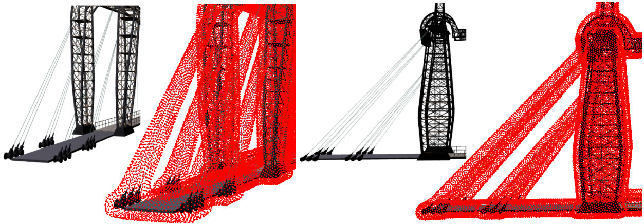
Figure 3.15: Pointshell for thin structures (e.g., cables): First and third image from left: the bridge geometry, viewed from two camera angles. Second and fourth image: the pointshell. Each red dot is one point. Points are fitted onto a level set (offset surface) of an unsigned distance field to the bridge geometry. Distance field resolution was 256 \times 256 \times 256 for this pointshell, and offset distance was 1.4 \times the size of a distance field voxel.
