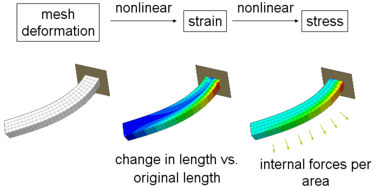
Figure 2.1: A deflected cantilever beam: Left: the deformed shape, Middle: strain, Right: stress. Both strain and stress are rank-2 tensors ( 3 \times 3 matrices for all practical purposes in this thesis); the plotted color gives the maximum eigenvalue of the 3 \times 3 matrix.
