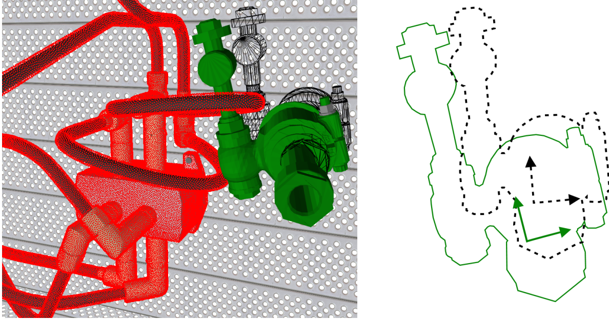
Figure 3.5: Virtual coupling: Left: the green mechanical component (distance field haptic object) and the deformable hose scene (pointshell, with points shown in red). Wireframe shows the manipulandum position, solid green color shows the simulation object position. Right: a schematic representation of the manipulandum position (stippled black line) and simulation position (solid green line), together with the two coordinate systems which virtual coupling tries to align.
