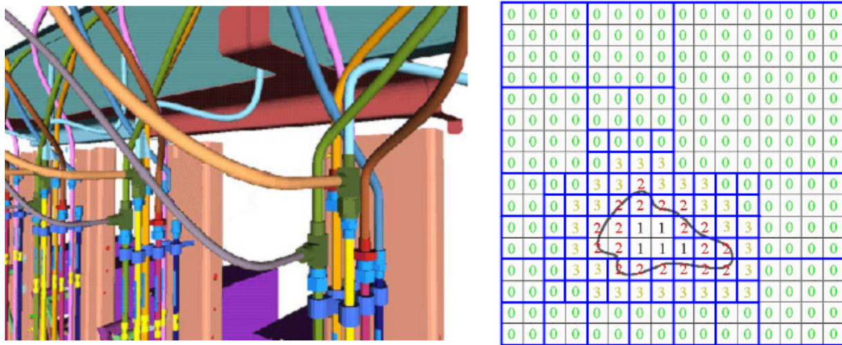
Figure 3.3: VPS voxmap : Left: a VPS environment (a scene from the interior of an airplane, serving as source data for voxmap). Right: a schematic illustration of the voxmap, also showing the voxmap octree. Both images are from [MPT99].
