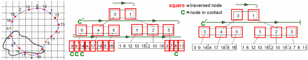
Figure 3.20: Graceful degradation: Left, Middle: With involved contact scenarios, many tree nodes need to be traversed during a complete hierarchy traversal. Right: Under graceful degradation, tree is traversed only up to a shallow depth, as permitted by available CPU power.
