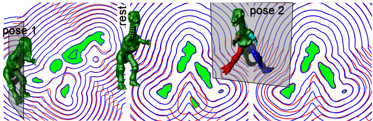
Figure 3.24: Isocontours of the exact and approximate deformed distance field: Left: Pose 1, single-domain approximation. Middle: Pose 2, single-domain approximation with the two legs mirroring. Right: Pose 2, multiple domain approximation without mirroring. Green denotes the interior of the object, with respect to the approximated field.
