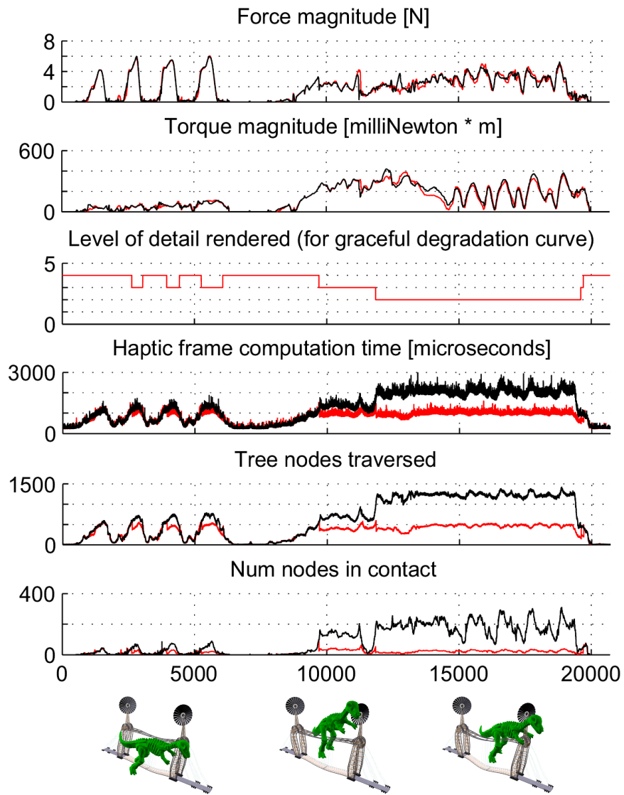
Figure 3.27: Illustration of graceful degradation (GD) : Simulation data for a pre-recorded manipulandum trajectory is rendered in two ways: using GD (in red) with warm threshold at 600 nodes; without GD (in black) with all four tree levels. The pointshell has 85,018 points total (same L4 pointshell as in Figure 3.15 on page 121). The common x -axis corresponds to haptic frames. This data was recorded on a three-year-old 3.0 GHz dual Intel Xeon processor with 2.75 Gb of memory, illustrating algorithm’s adaptivity to different computer speeds. On the machine of Table 3.1, the black timing curve reaches a maximum of \sim 800 \mu s .
