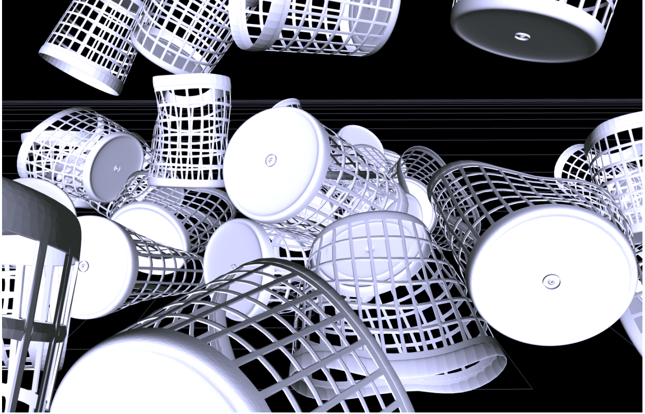
Figure 2.16: Multibody dynamics simulation with large deformations: In this simulation, we dropped 512 flexible baskets to the ground. The baskets started from zero velocity, horizontally separated (but in close proximity) at a certain height. Collision detection was performed using a BD-Tree [JP04]. Penalty forces were applied between leaf spheres to resolve contact. Motion basis ( r = 40 ) used linear modes \Psi_7, \dots, \Psi_{26} and their derivatives. The rigid body motion was not coupled with deformations, although this would not be a difficult extension [Sha05]. It took 1.2 sec total to perform the 512 implicit Newmark steps to advance the reduced deformations to the next graphical frame.
