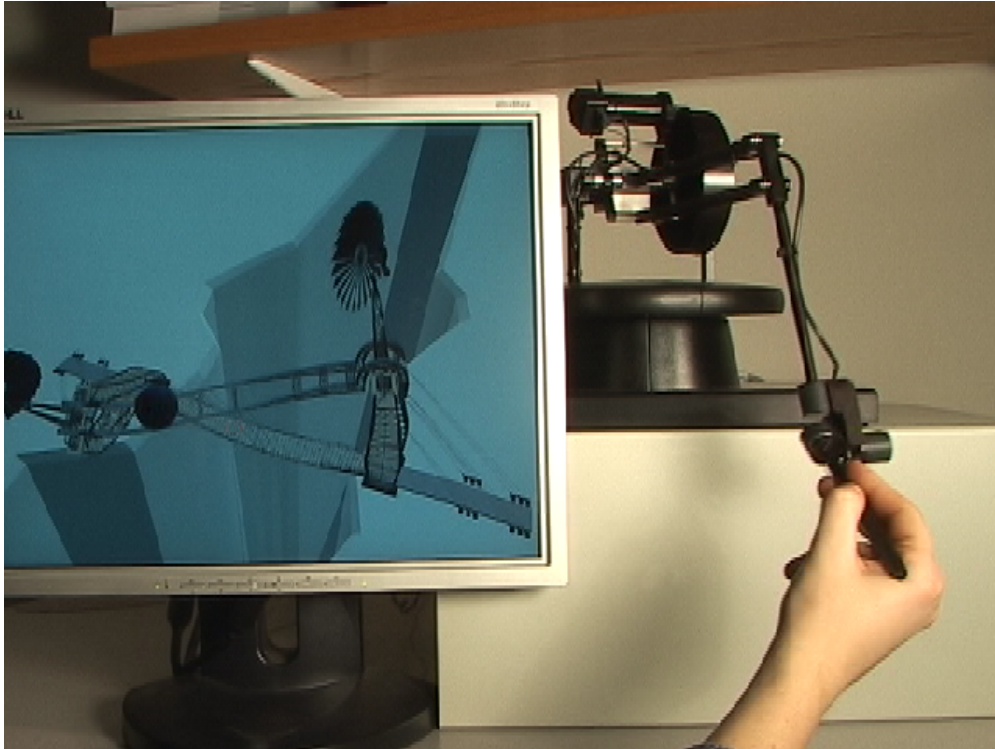
Figure 1.2: Large-deformation dynamics at kilohertz rates are a key ingredient of deformable haptic simulations. Note the large bridge deformation resulting from contact with a user-controlled ball. Bridge is simulated in a 15-dimensional basis of deformations. Each timestep of the deformable object simulation took 65 microseconds to compute on a 3.0 Ghz Intel Pentium Xeon workstation with 2Gb of memory (manufactured in 2004).
