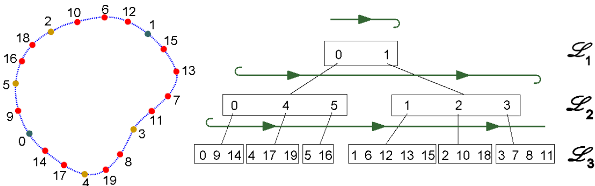
Figure 3.18: Nested point-tree: Left: The pointshell. Right: the hierarchy, the traversal order and tree levels \mathcal{L}_i . Particle-repulsion levels are 0-1, 2-5, and 6-19 in this case.
