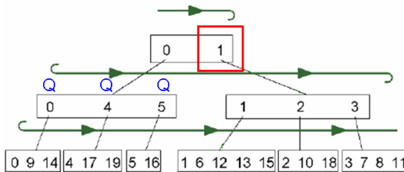
Figure 3.19: Tree traversal: Left: The bounding sphere of node 0 intersects the environment and all the children are queued for traversal (indicated by the symbol 'Q'). Right: Node 1 is sufficiently far from contact that its bounding sphere does not intersect the environment, and as such, the subtree need not be traversed further. This completes the traversal of Level 1. The traversal list for Level 2 is \{0, 4, 5\} , where 0 is in this case the copy on level 2.
