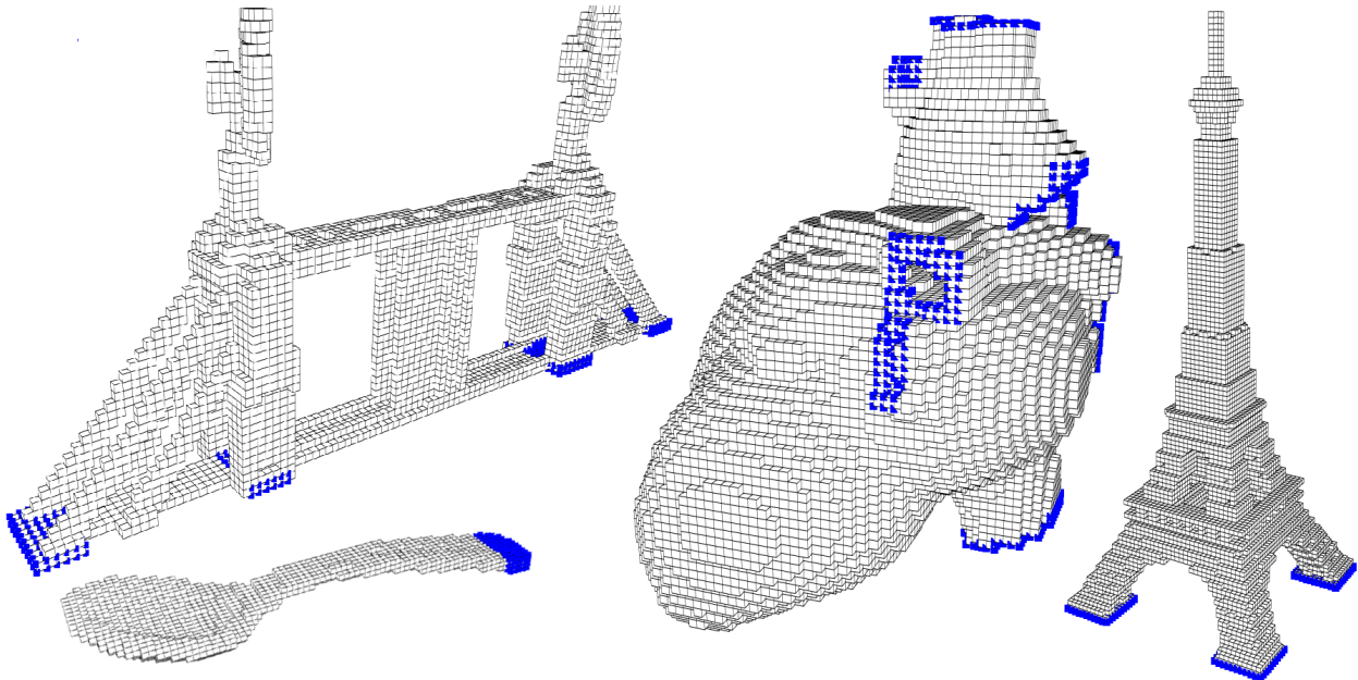
Figure 2.6: Simulation Meshes: Blue vertices are constrained.
