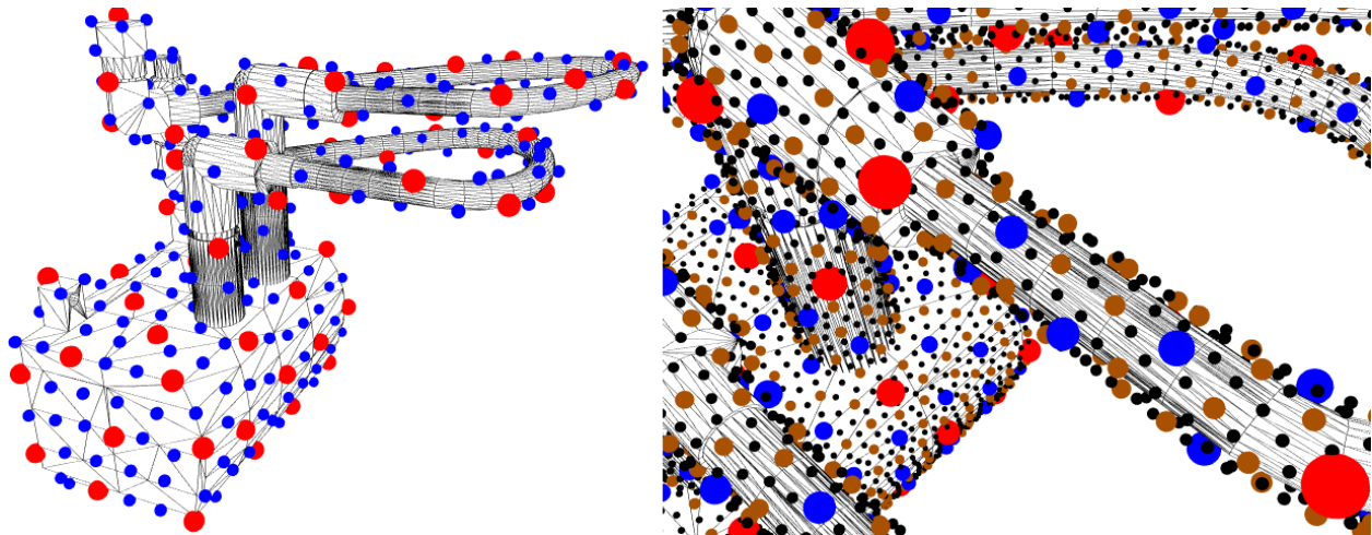
Figure 3.14: Multi-resolution oriented pointshell from particle repulsion: Left: The first two levels of a part of the hose scene. Right: detail with four levels shown. Points are fitted on a small-distance offset oriented manifold surface to support “polygon soup” input geometry, and provide oriented surface normals for contact.
