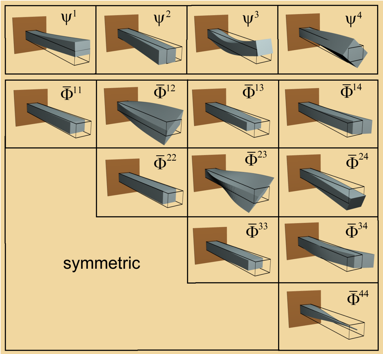
Figure 2.13: Dominant linear modes and modal derivatives: We exploit the statistical redundancy of these modes using mass-PCA of suitably scaled modes. All vectors are shown mass-normalized.
