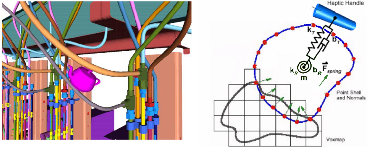
Figure 3.4: VPS in action: Left: the user manipulates the teapot in the virtual environment. Right: the virtual coupling between the haptic device and the manipulated simulation object in contact. Both images are from [MPT99].
