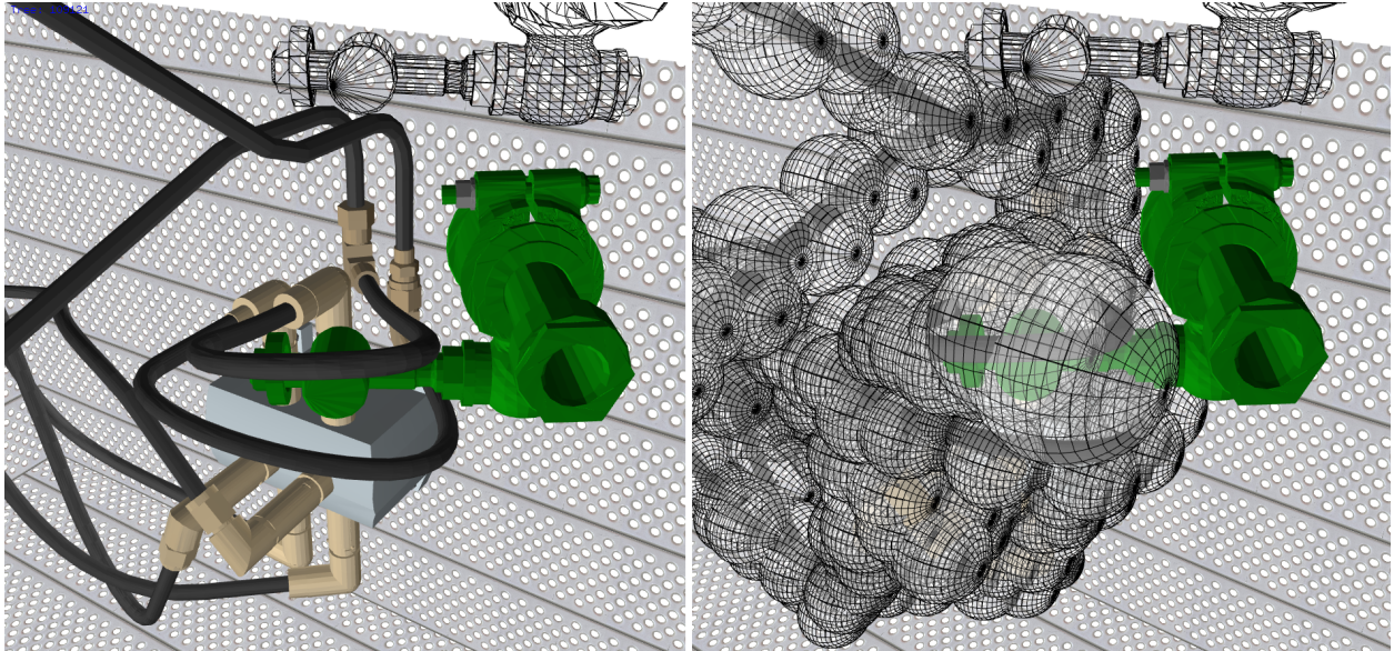
Figure 3.12: Point-based BD-Tree performance under large deformations: The sphere radii do grow under large deformations (see, e.g., two level-1 spheres at the tip of the upper u-shaped hose), however tree traversal is still very efficient. The upper hose is bent at an angle of approximately 25 degrees. If the green part is lowered (but kept inserted in between hoses) such that the upper hose returns to (almost) rest configuration, the performance changes from 220\mu s to 210\mu s . To the best of our knowledge, while limited to reduced deformations (as in our case), BD-Tree is the only deformable bounding volume hierarchy update method that can reach haptic update rates (1000 Hz) with example complexity similar to ours. In general, the BD-Tree performs especially well when large deformations are localized to a part of the scene; also, BD-Tree could be augmented by computing bounds at configurations other than the rest configuration.
