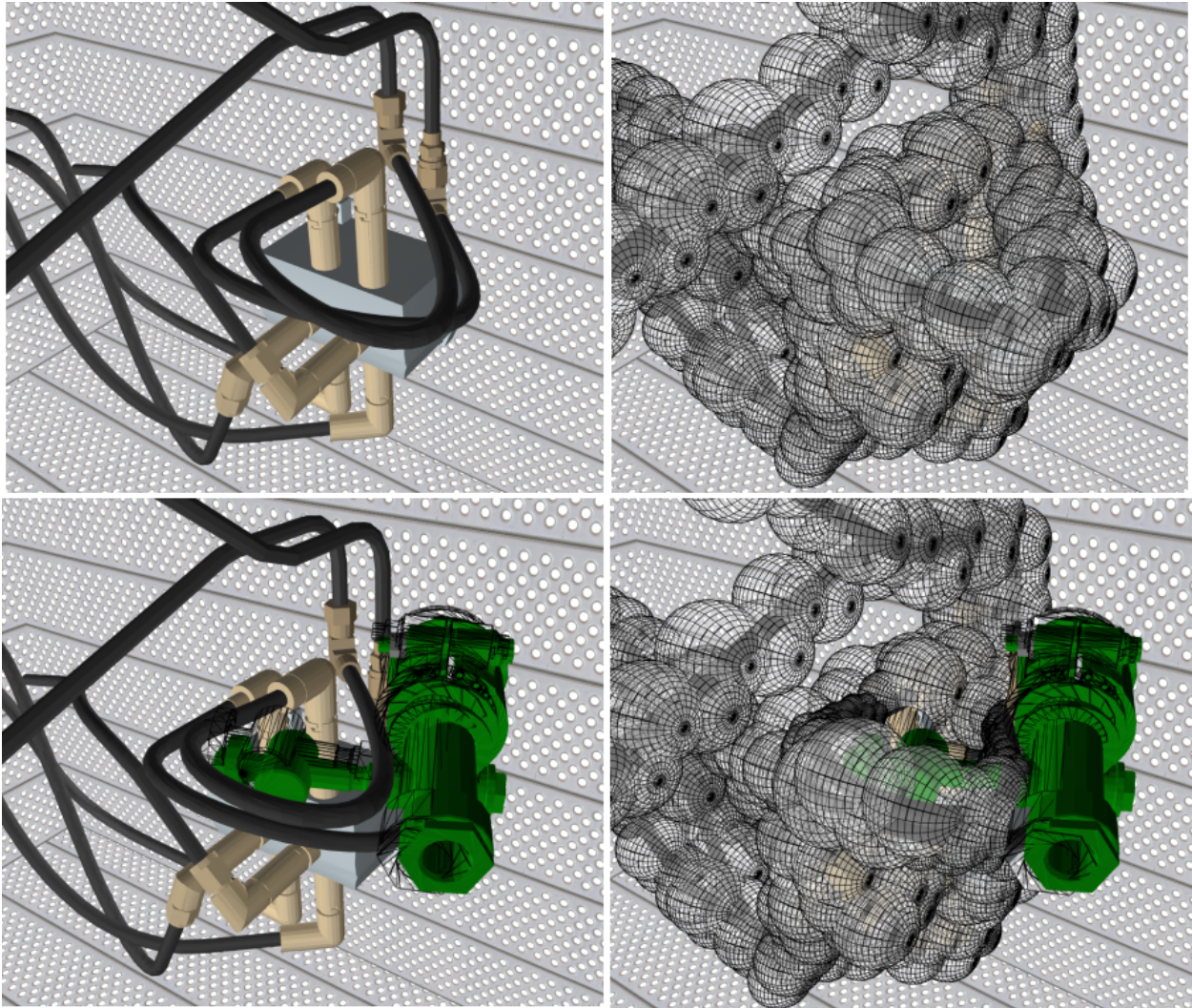
Figure 3.11: Point-based BD-Tree: Top row: the rest configuration. Bottom row: tree during contact. Right column shows the deepest bounding spheres that were traversed during this particular haptic cycle (i.e., each rendered sphere is free of contact). Note how the tree is traversed to different depths depending on proximity to contact. We typically use many spheres (320 in this example) on the first level, followed by 4x more spheres on consecutive levels. First-level spheres are always traversed (therefore they appear in top-right image) if temporal coherence is off; however, when temporal coherence is enabled most of them need not actually be checked during most haptic cycles. There are 4 hierarchy levels in this example. The small spheres next to the green metallic part in the bottom-right image are level 3 spheres. Level 4 spheres have zero radius, as they correspond to leaf points.
