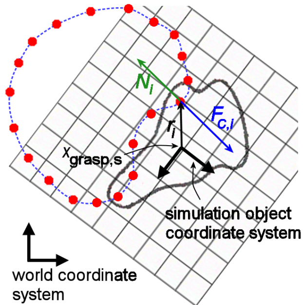
Figure 4.3: The contact model
