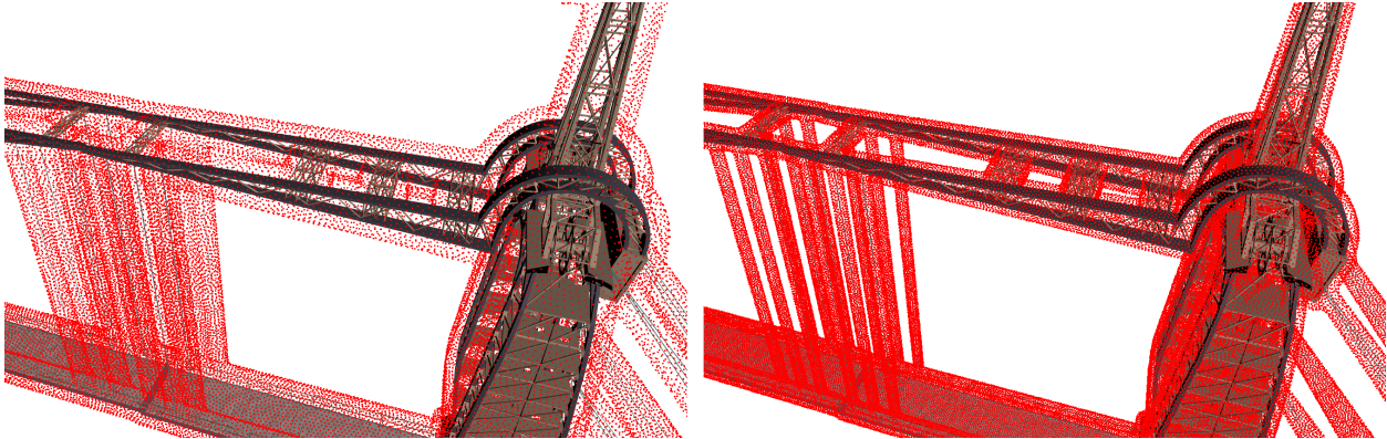
Figure 3.16: Pointshell for thin structures with a smaller offset: Left: pointshell (four levels, 85,000 points) fitted using a 256 \times 256 \times 256 unsigned distance field (same pointshell as in Figure 3.15). Right: pointshell (five levels, 256,000 points) fitted using a 512 \times 512 \times 512 unsigned distance field, and with a 2x smaller offset distance as pointshell on the left. Both pointshells use an offset of 1.4x the size of the distance field voxel. Note that the finer pointshell resolves all twelve central vertical cables on the bridge, whereas the coarser pointshell merges groups of three cables together. Simulation with the finer pointshell is more permissive (accurate) in that thicker objects can be inserted through holes in pointshell geometry, such as the holes in the bridge’s upper shelf. In general, higher resolution unsigned distance fields are required for smaller offsets, otherwise the offset surface becomes progressively non-smooth (noisy).
