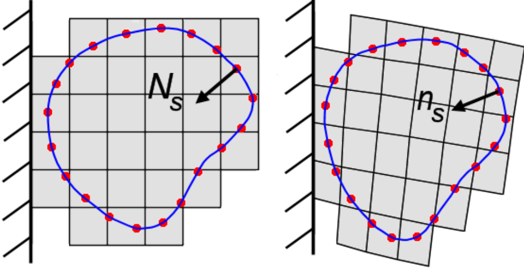
Figure 3.8: (Inward) normals deformed with deformation gradients: Left: undeformed configuration. Right: deformed configuration. Our pointshell surfaces are embedded into FEM volumetric meshes (voxel volumetric mesh is shown in gray). Volumetric mesh deformations drive the pointshell point positions and normals.
