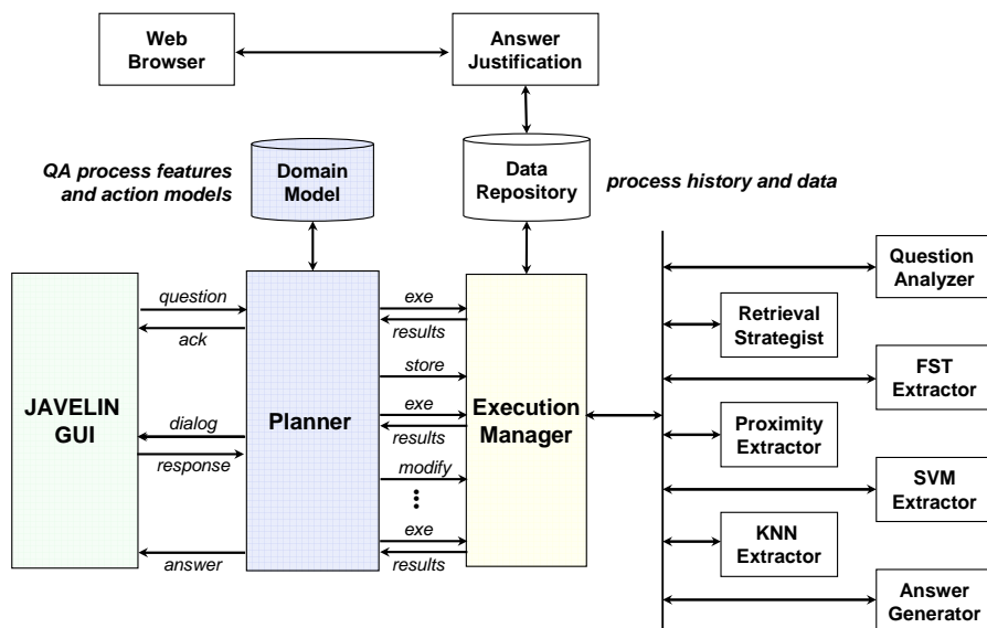
Figure 1: The JAVELIN QA architecture.
