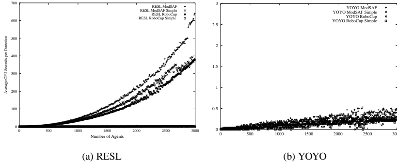
Figure 2: Comparing YOYO to RESL. The X axis marks the number of agents monitored; the Y axis denotes computation time in CPU seconds. Note (a) and (b) have different ranges on the Y axis.
