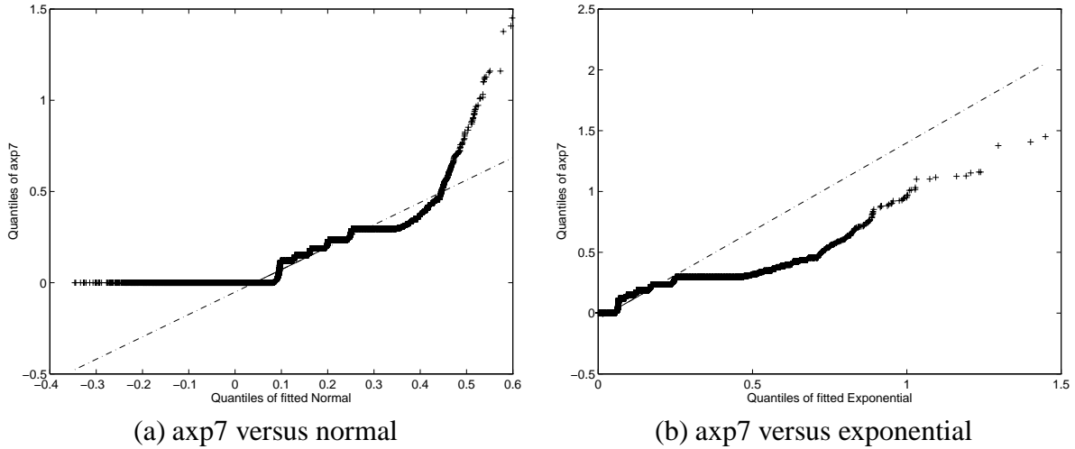
Figure 7: Quantile-quantile plots for axp7 trace of August 19, 1997.
