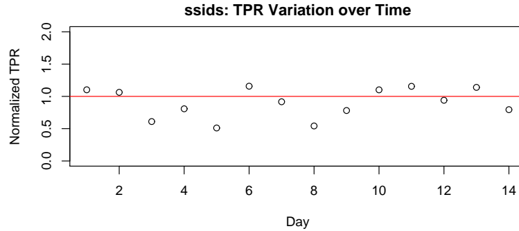
Figure 2.6: Accuracy over time. Normalized mean TPR on each day in the apt trace for FPR = 0.01. Each TPR value is normalized to the mean TPR for the entire period, evaluated over the users present during that day. The mean TPR for the entire period over all profiled users is 42%.
