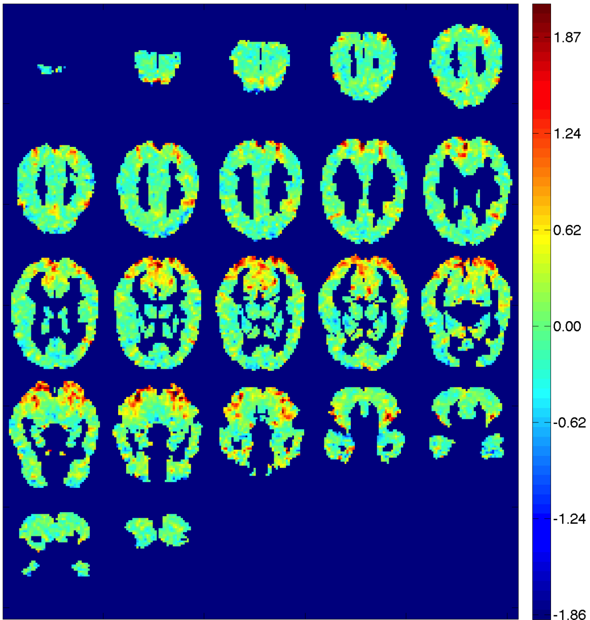
Figure 2.4: An fMRI image averaged over 6 repetition of a person reading the word “bear”. An fMRI image is 3D, here shown in slices progressing from the top of the head (top left) to the bottom of the head (bottom right). In each slice, the front of the head points towards the bottom of the figure, and the right side of the subject is shown on the left side of the each image (as if we are viewing the brain of a subject laying face down, from the top of their head). The color of each voxel (pixel in brain space) represents the percent change over baseline of the BOLD response in that brain area.
