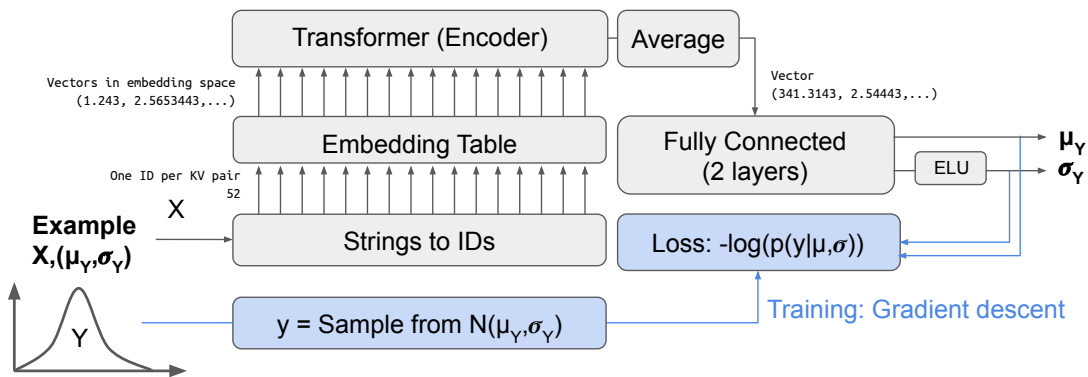
(c) Embedding-based Transformer
