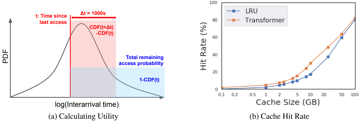
Figure 3.8: Using predictions in caching.
