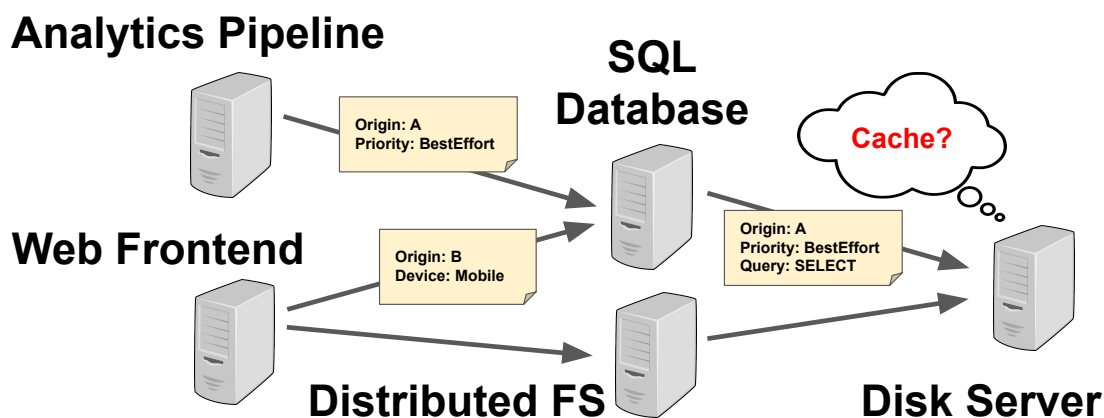
Figure 3.2: Census tags are free-form key-value pairs that are added by services and propagated with subsequent requests.
