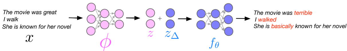
Figure 4.1: vec2text models (consisting of a fixed embedding model \phi and a learned decoder model f_\theta ) can be used to perform various transformations of inputs (e.g., changing tense) reasonably reliably by applying simple arithmetic operations to latent vectors.
