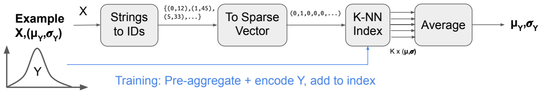
(b) Nearest Neighbor Model
