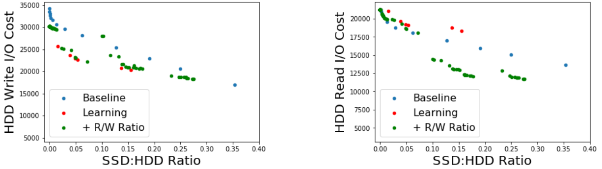
Figure 3.9: Using predictions in SSD/HDD tiering.
